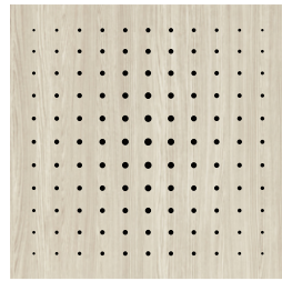
01 ø2.5-15.5 dots 50mm spacing
