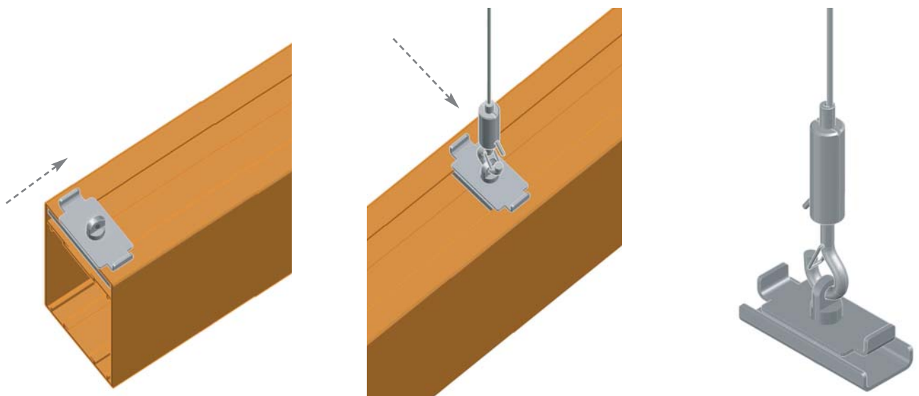
Fig 2. Locating the Clamping Bracket in the 50mm Beam
