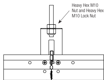
PMHC – Prelude Max Hanging Clip
