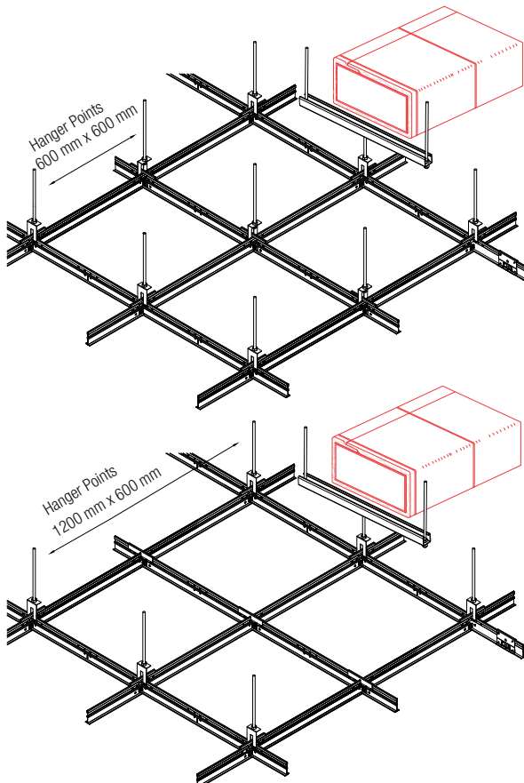
PMHC – Prelude Max Hanging Clip
