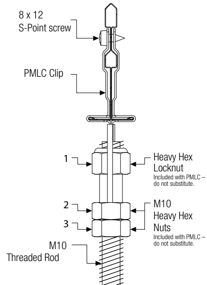
Load Connector Clip Installation
