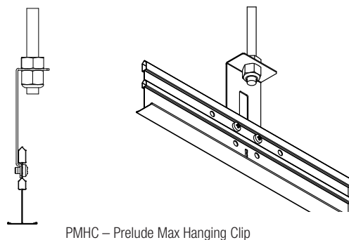
PMHC – Prelude Max Hanging Clip
